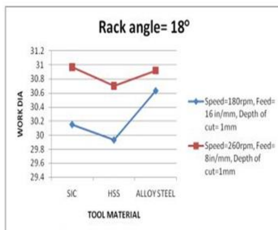
Figure.3. Effect of tool impact with rake angle 18°
