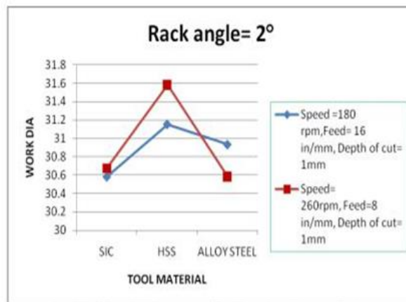
Figure.1. Effect of tool impact with rake angle 2°
