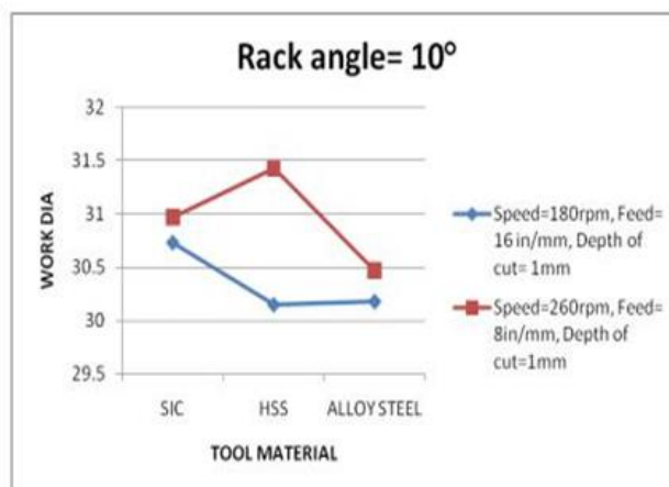
Figure.2. Effect of tool impact with rake angle 10°
